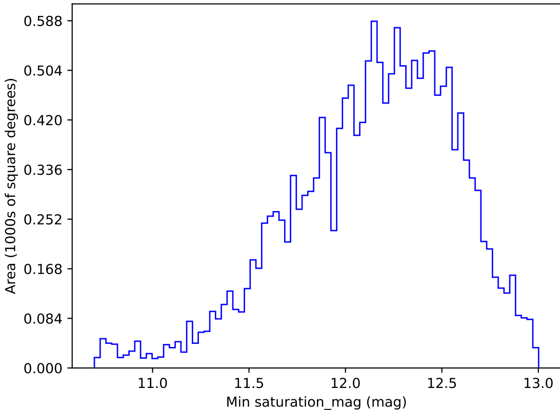
early_u_fpextra3.0_v3.4_10yrs WFD z band: Min saturation_mag
