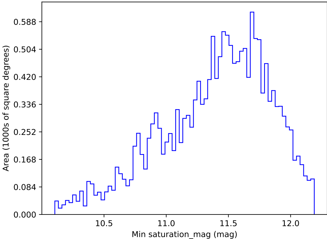
early_u_fpextra3.0_v3.4_10yrs WFD u band: Min saturation_mag
