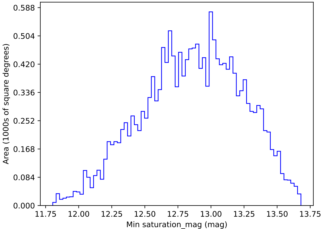
early_u_fpextra3.0_v3.4_10yrs WFD g band: Min saturation_mag
