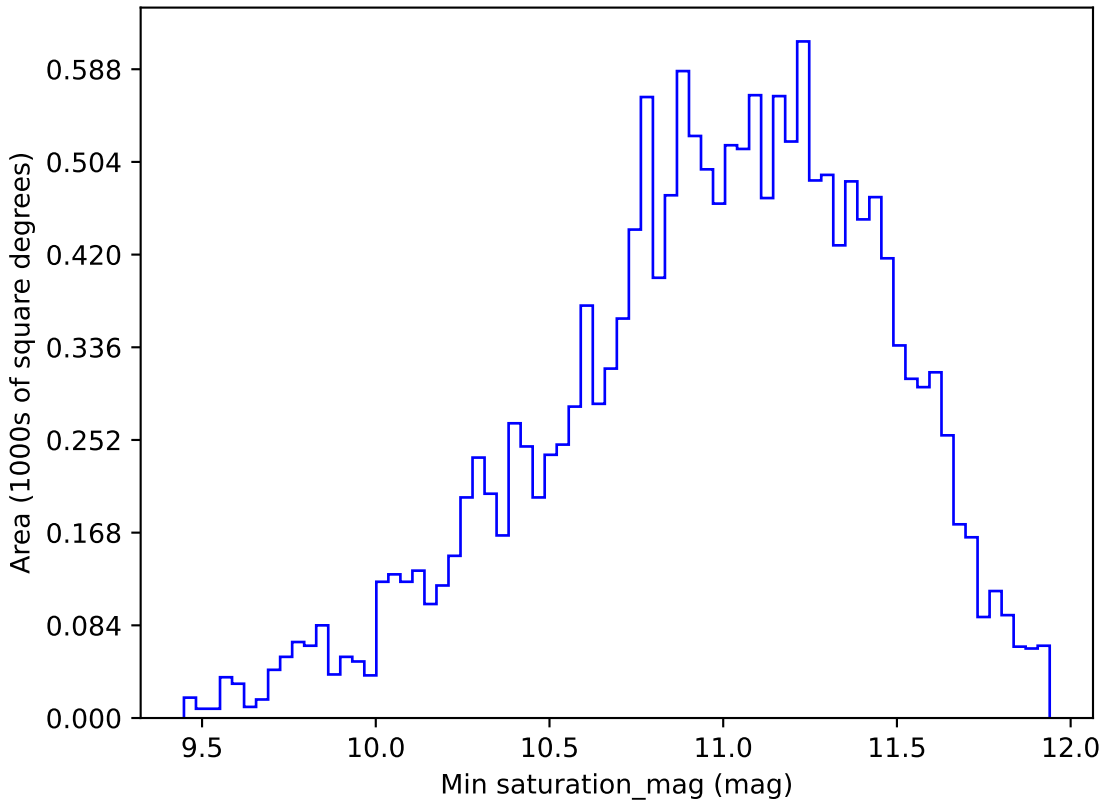
early_u_fpextra3.0_v3.4_10yrs WFD all bands: Min saturation_mag
