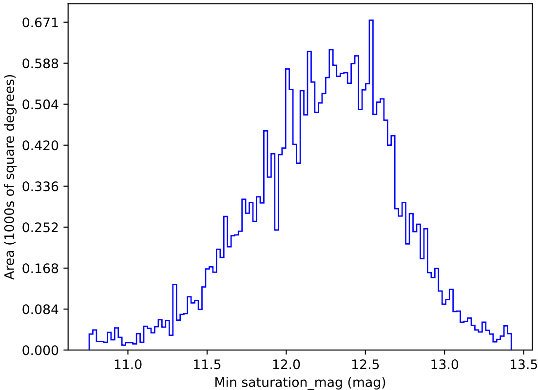
early_u_fpextra3.0_v3.4_10yrs All sky z band: Min saturation_mag
