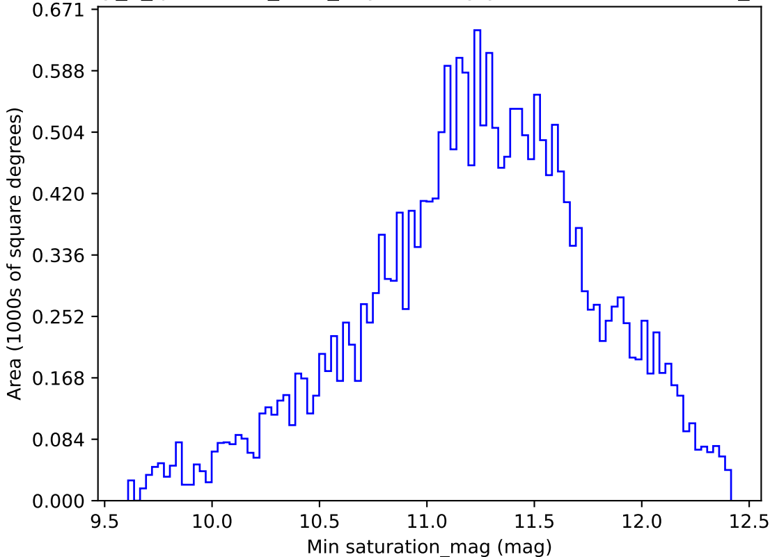
early_u_fpextra3.0_v3.4_10yrs All sky y band: Min saturation_mag
