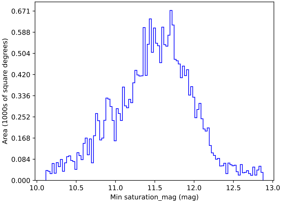
early_u_fpextra3.0_v3.4_10yrs All sky u band: Min saturation_mag
