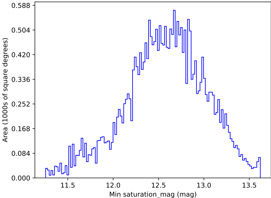
early_u_fpextra3.0_v3.4_10yrs All sky r band: Min saturation_mag
