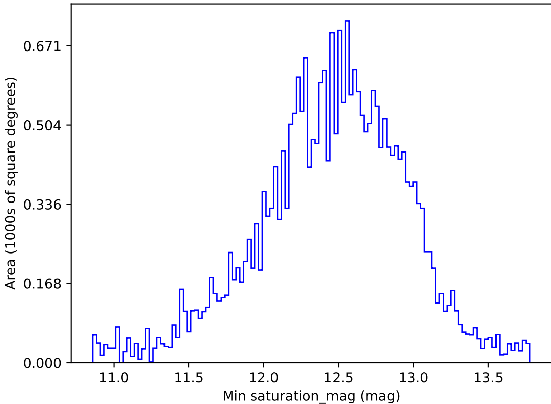
early_u_fpextra3.0_v3.4_10yrs All sky i band: Min saturation_mag
