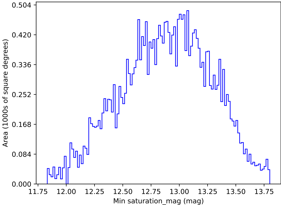
early_u_fpextra3.0_v3.4_10yrs All sky g band: Min saturation_mag
