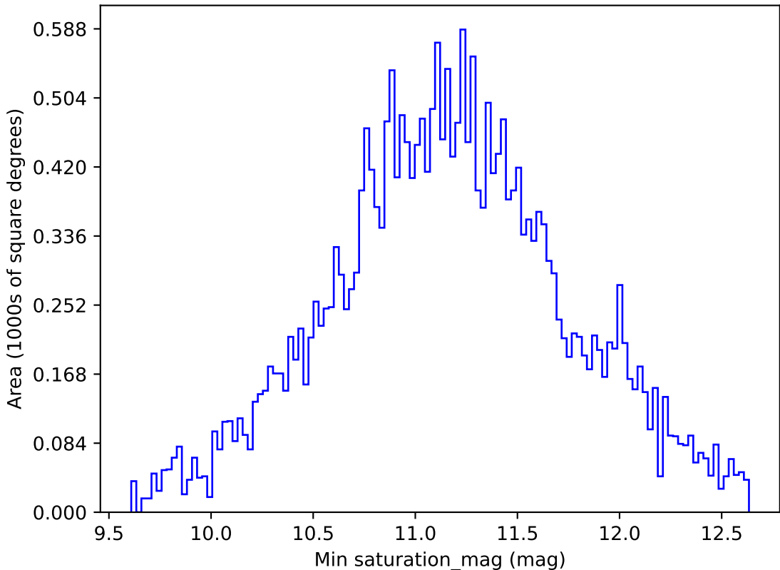
early_u_fpextra3.0_v3.4_10yrs All sky all bands: Min saturation_mag
