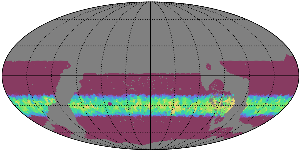
early_u_fpextra3.0_v3.4_10yrs WFD y band: Min normairmass
