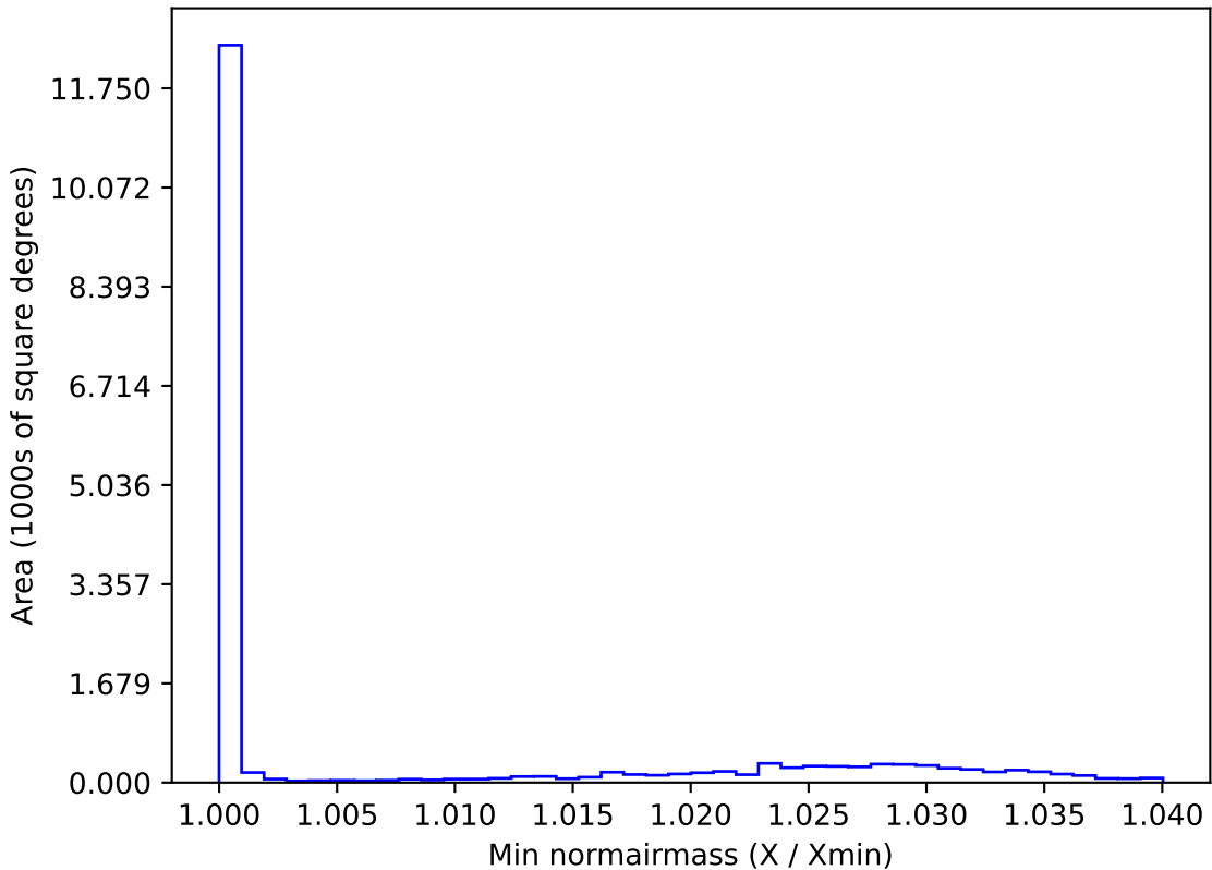
early_u_fpextra3.0_v3.4_10yrs WFD y band: Min normairmass
