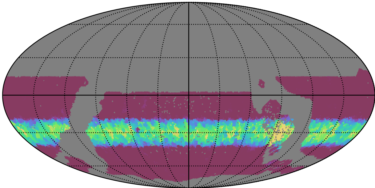
early_u_fpextra3.0_v3.4_10yrs WFD u band: Min normairmass
