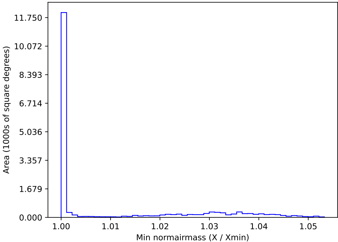
early_u_fpextra3.0_v3.4_10yrs WFD u band: Min normairmass
