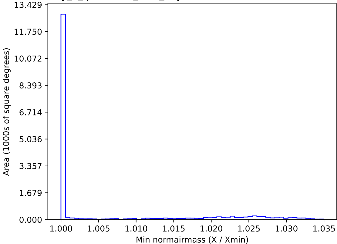
early_u_fpextra3.0_v3.4_10yrs WFD r band: Min normairmass
