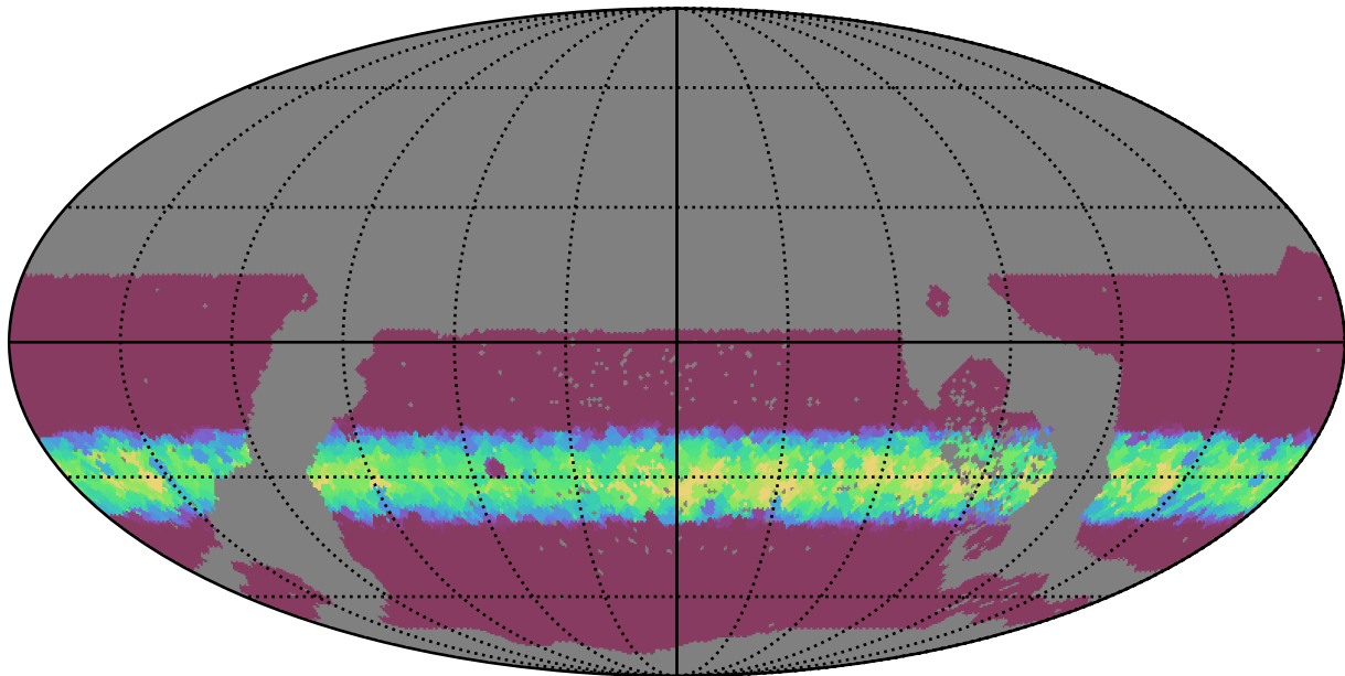
early_u_fpextra3.0_v3.4_10yrs WFD i band: Min normairmass
