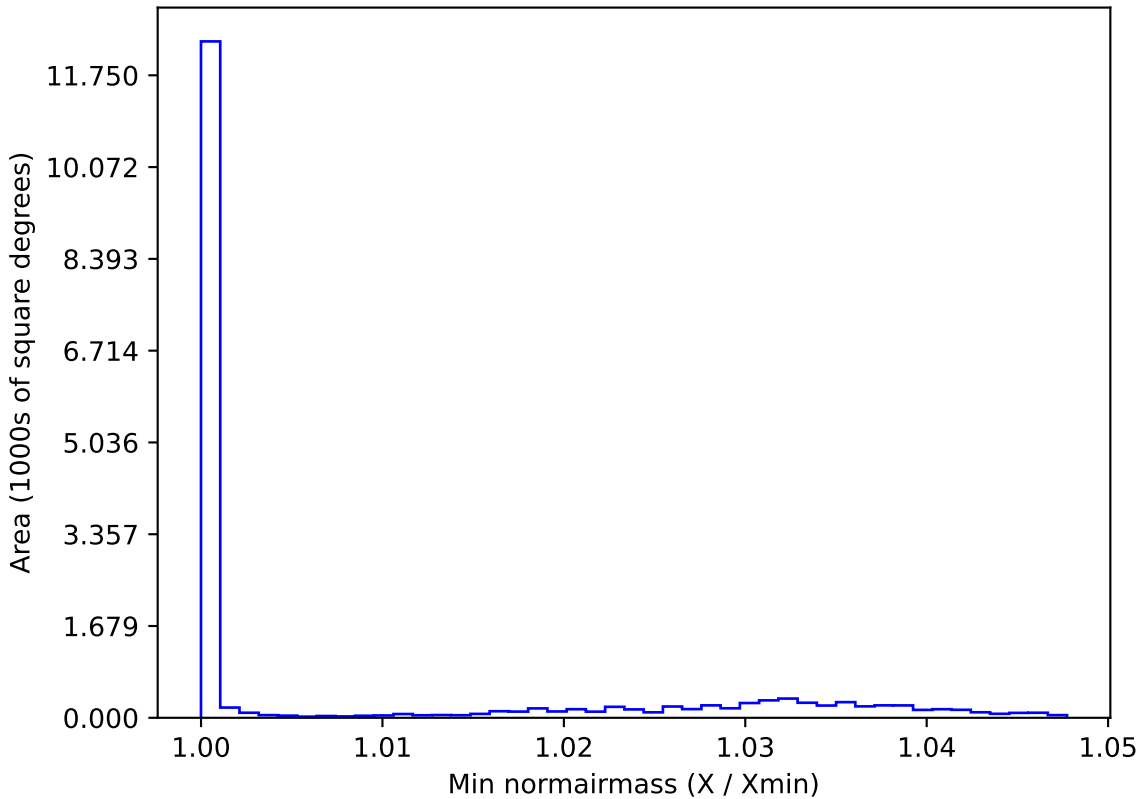
early_u_fpextra3.0_v3.4_10yrs WFD g band: Min normairmass
