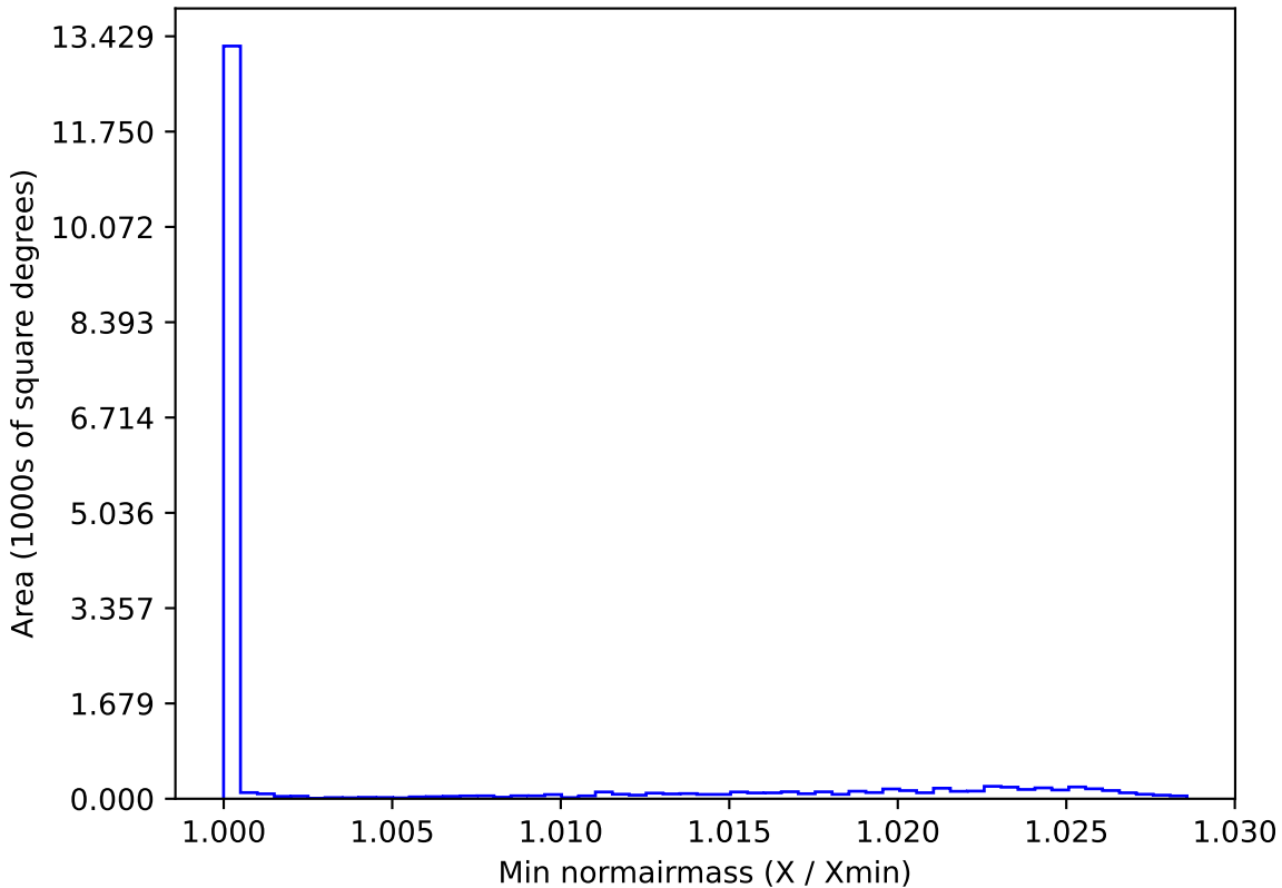
early_u_fpextra3.0_v3.4_10yrs WFD all bands: Min normairmass
