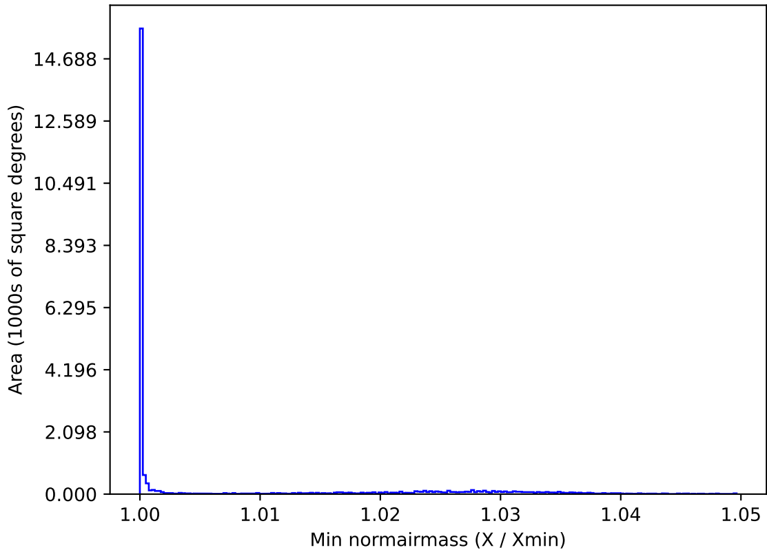
early_u_fpextra3.0_v3.4_10yrs All sky y band: Min normairmass
