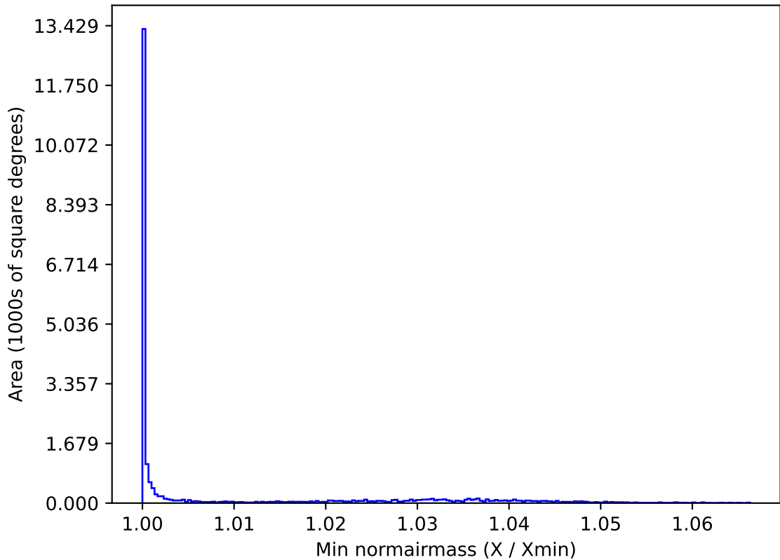
early_u_fpextra3.0_v3.4_10yrs All sky u band: Min normairmass
