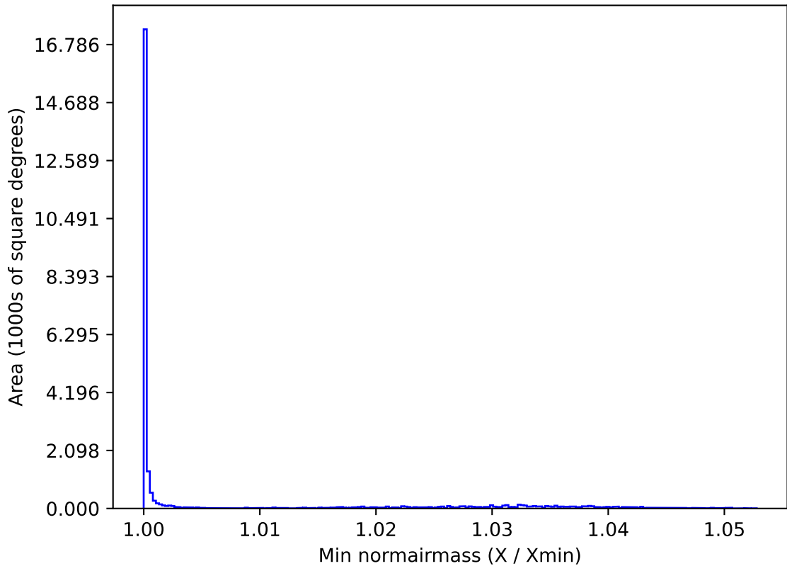
early_u_fpextra3.0_v3.4_10yrs All sky g band: Min normairmass
