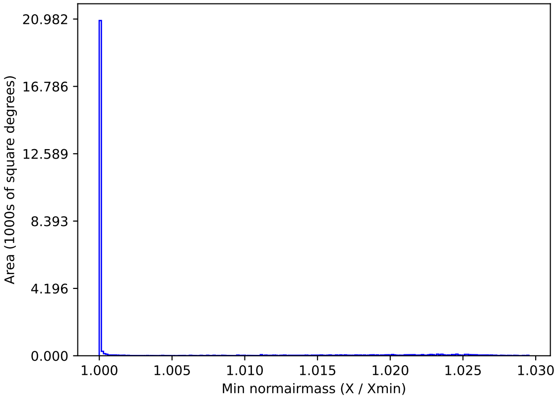
early_u_fpextra3.0_v3.4_10yrs All sky all bands: Min normairmass
