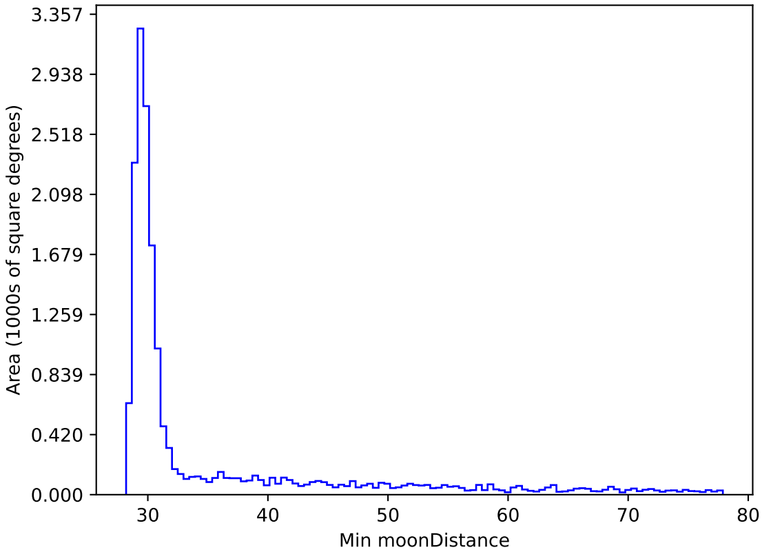
early_u_fpextra3.0_v3.4_10yrs WFD z band: Min moonDistance
