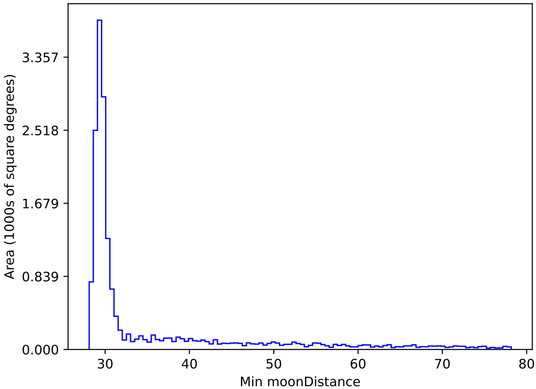
early_u_fpextra3.0_v3.4_10yrs WFD y band: Min moonDistance
