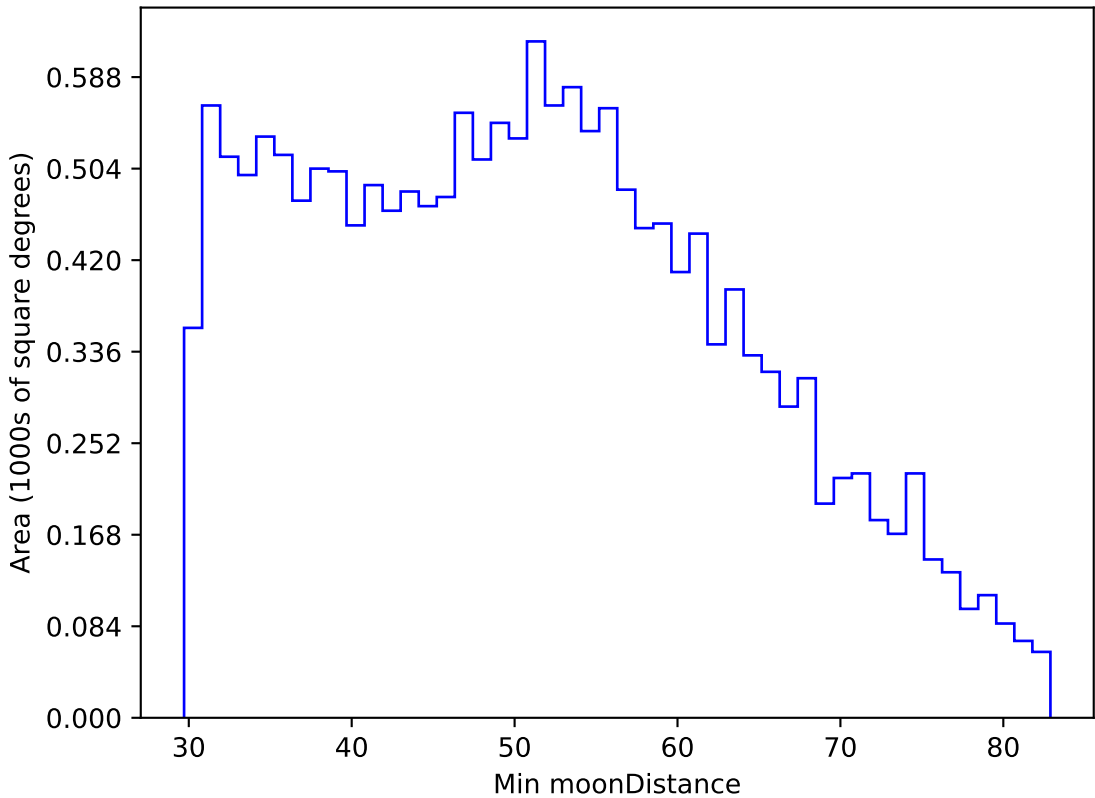
early_u_fpextra3.0_v3.4_10yrs WFD u band: Min moonDistance
