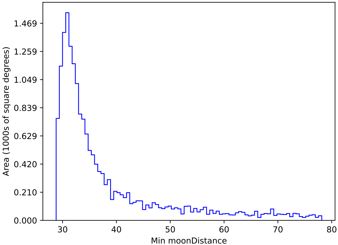
early_u_fpextra3.0_v3.4_10yrs WFD r band: Min moonDistance
