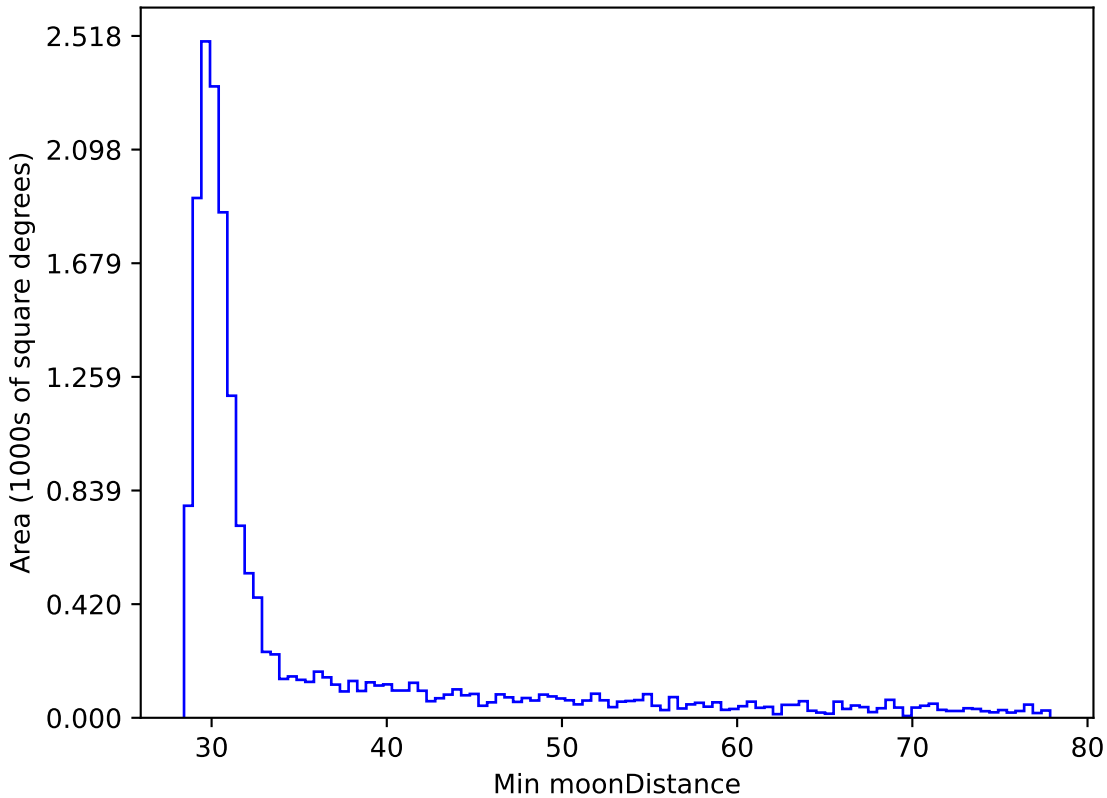
early_u_fpextra3.0_v3.4_10yrs WFD i band: Min moonDistance
