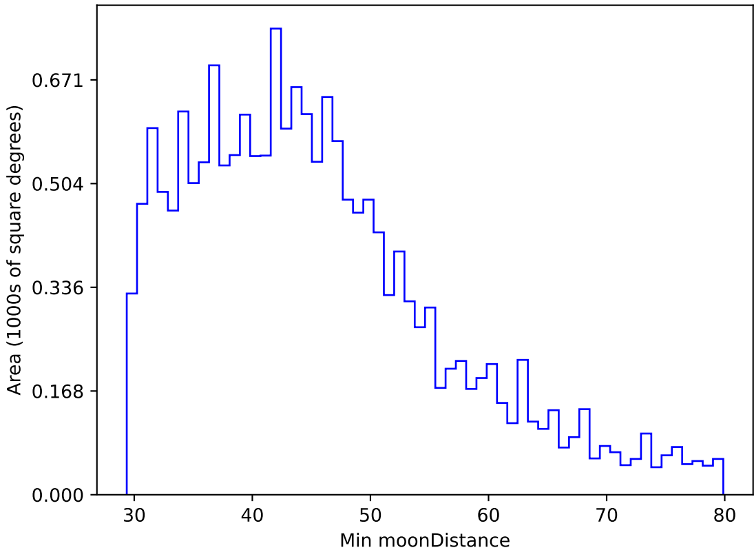
early_u_fpextra3.0_v3.4_10yrs WFD g band: Min moonDistance
