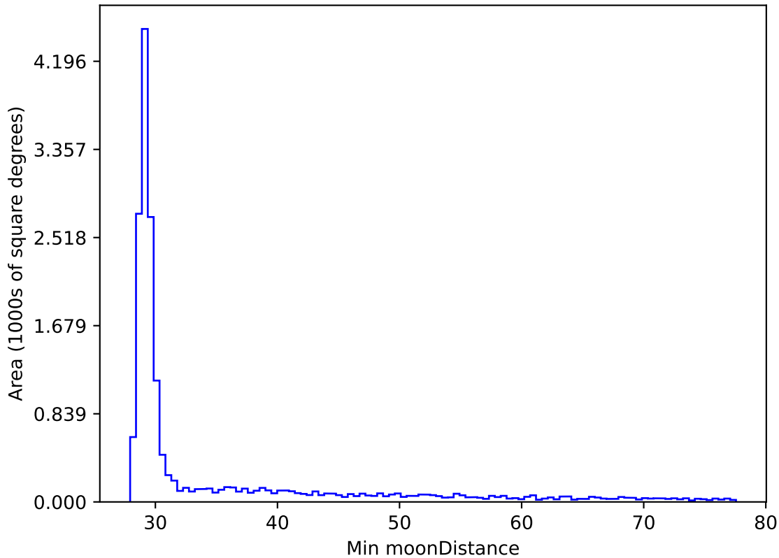
early_u_fpextra3.0_v3.4_10yrs WFD all bands: Min moonDistance
