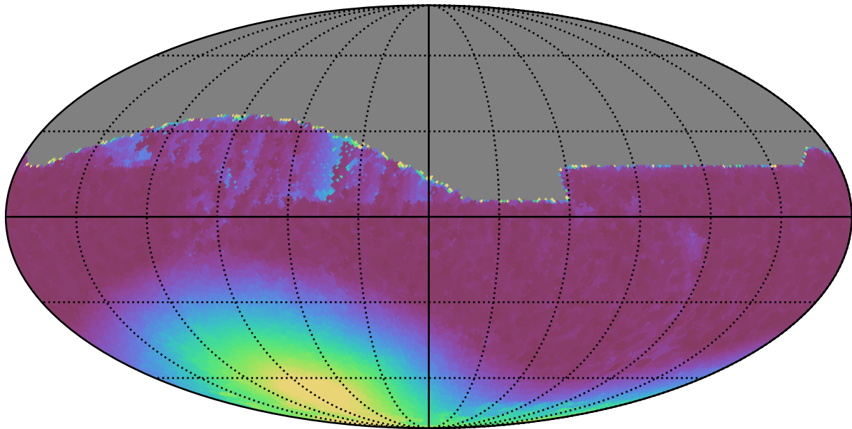
early_u_fpextra3.0_v3.4_10yrs All sky z band: Min moonDistance
