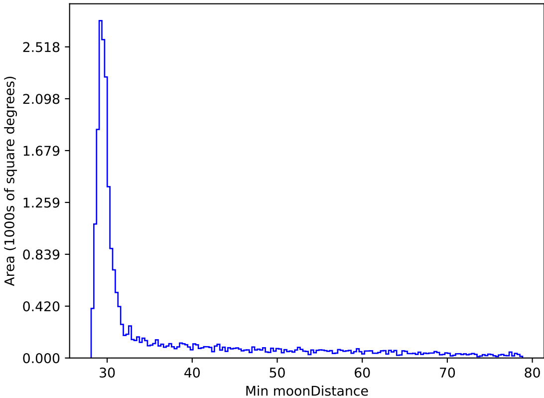
early_u_fpextra3.0_v3.4_10yrs All sky y band: Min moonDistance
