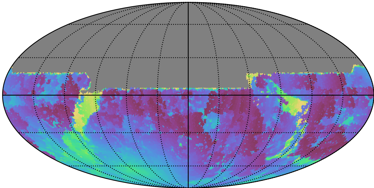
early_u_fpextra3.0_v3.4_10yrs All sky u band: Min moonDistance
