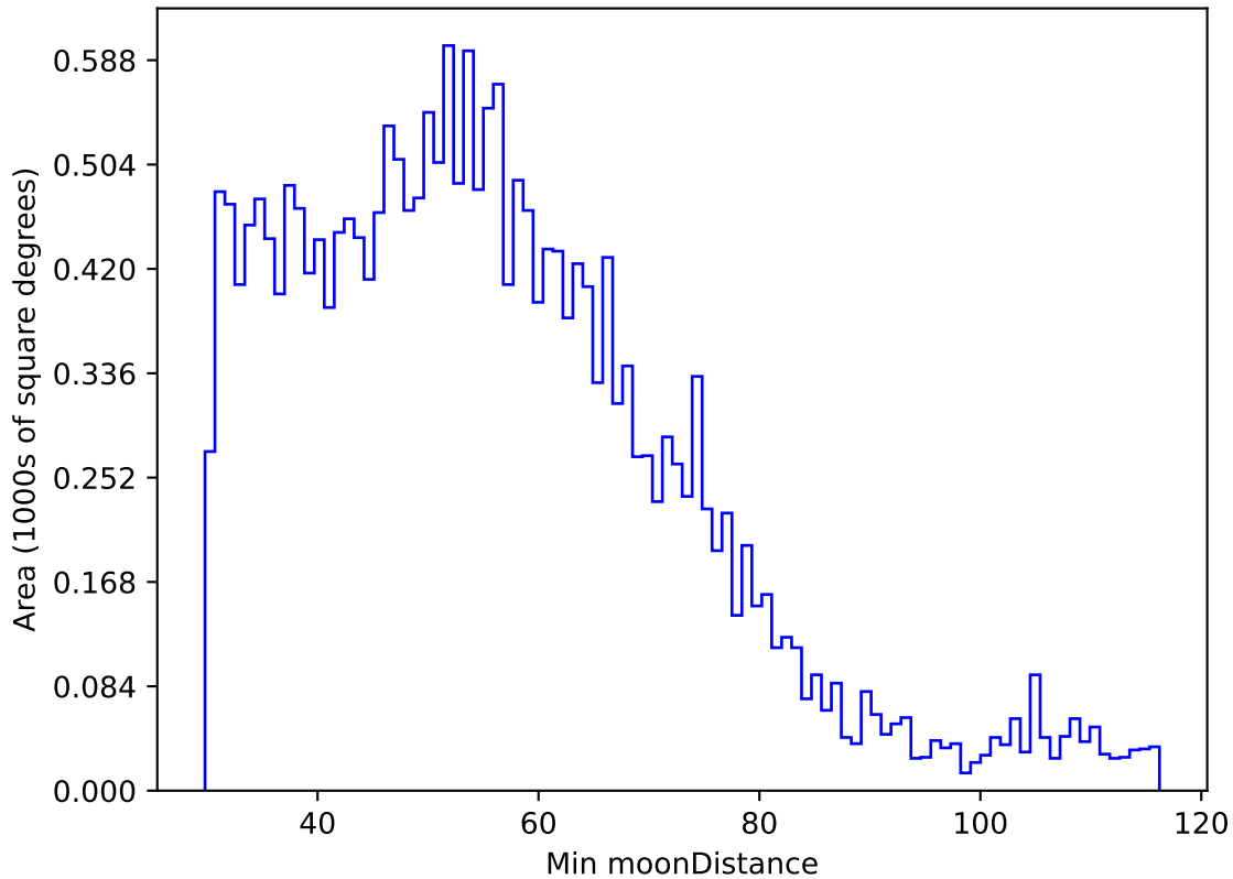
early_u_fpextra3.0_v3.4_10yrs All sky u band: Min moonDistance
