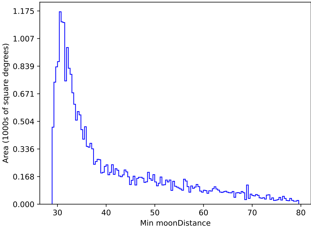
early_u_fpextra3.0_v3.4_10yrs All sky r band: Min moonDistance
