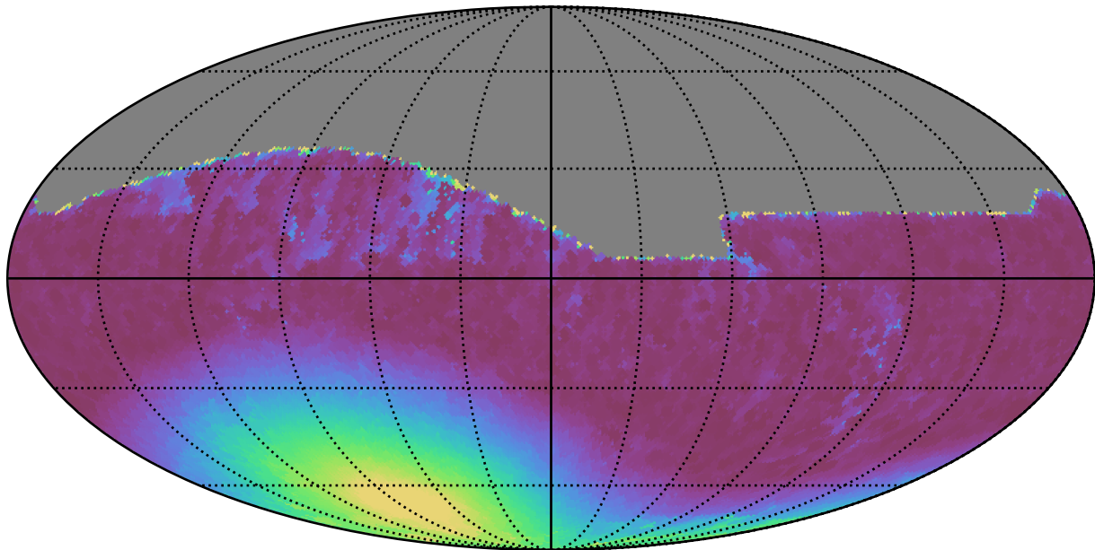
early_u_fpextra3.0_v3.4_10yrs All sky i band: Min moonDistance
