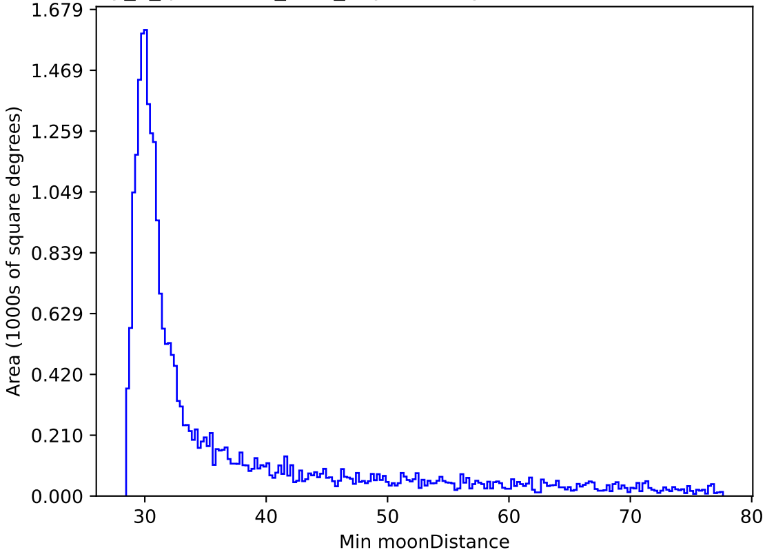
early_u_fpextra3.0_v3.4_10yrs All sky i band: Min moonDistance
