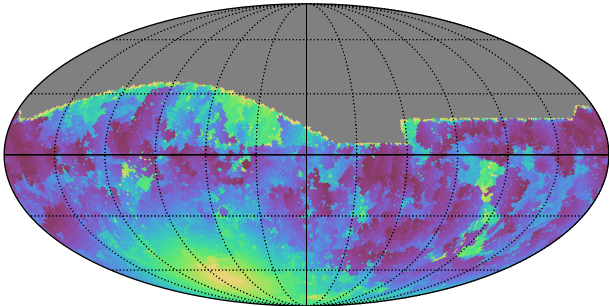
early_u_fpextra3.0_v3.4_10yrs All sky g band: Min moonDistance
