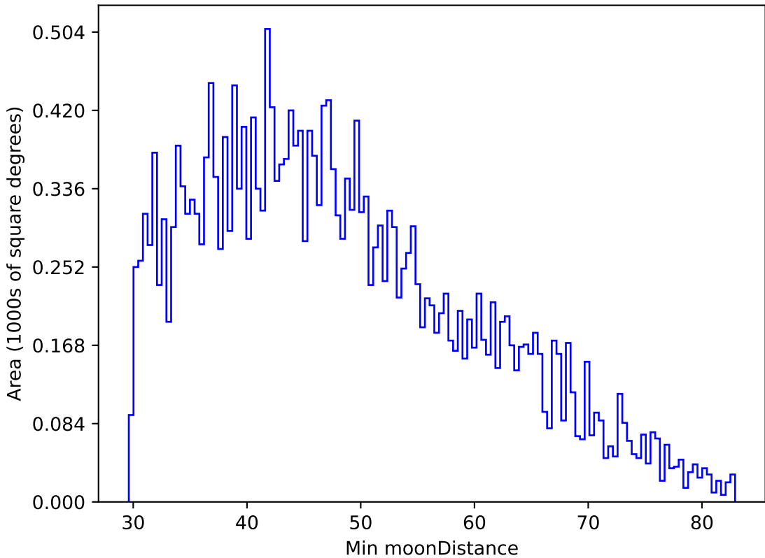
early_u_fpextra3.0_v3.4_10yrs All sky g band: Min moonDistance
