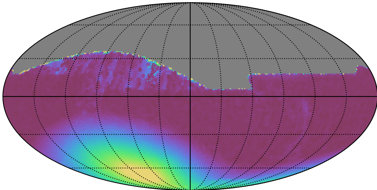
early_u_fpextra3.0_v3.4_10yrs All sky all bands: Min moonDistance
