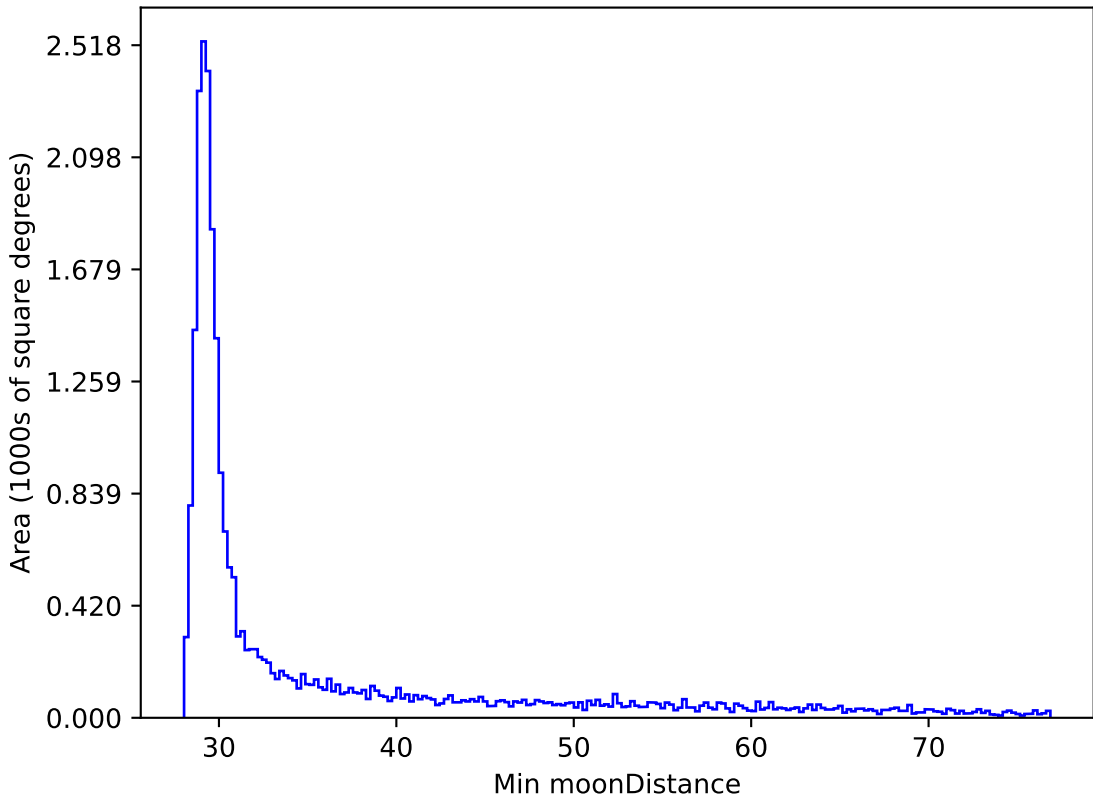
early_u_fpextra3.0_v3.4_10yrs All sky all bands: Min moonDistance
