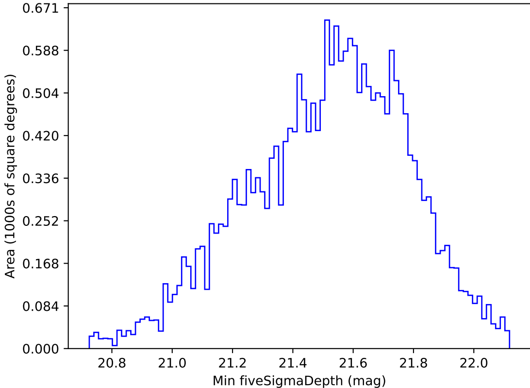
early_u_fpextra3.0_v3.4_10yrs Yr 1 y band: Min fiveSigmaDepth
