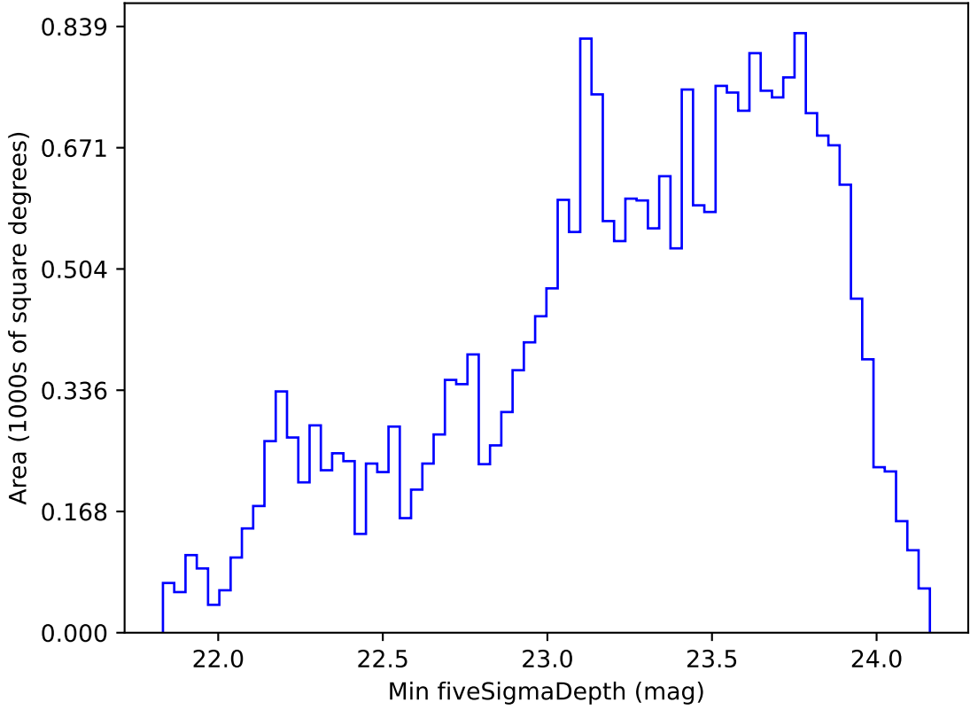
early_u_fpextra3.0_v3.4_10yrs Yr 1 r band: Min fiveSigmaDepth
