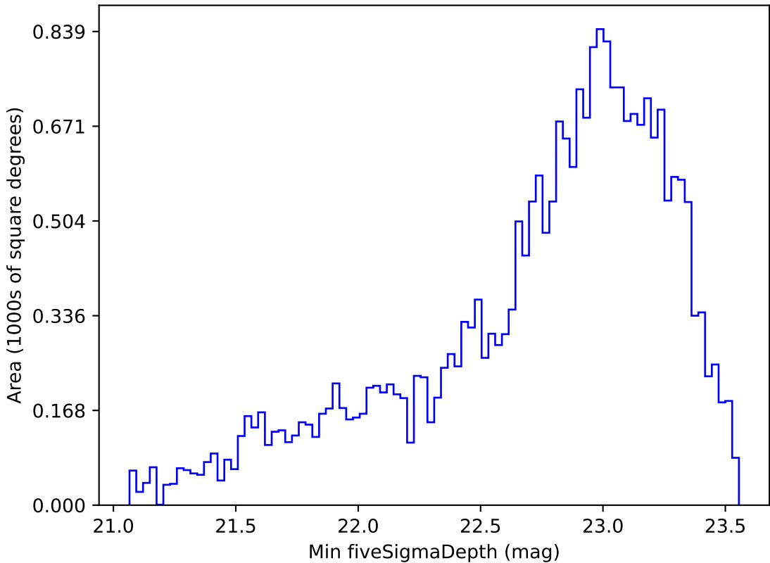
early_u_fpextra3.0_v3.4_10yrs Yr 1 i band: Min fiveSigmaDepth
