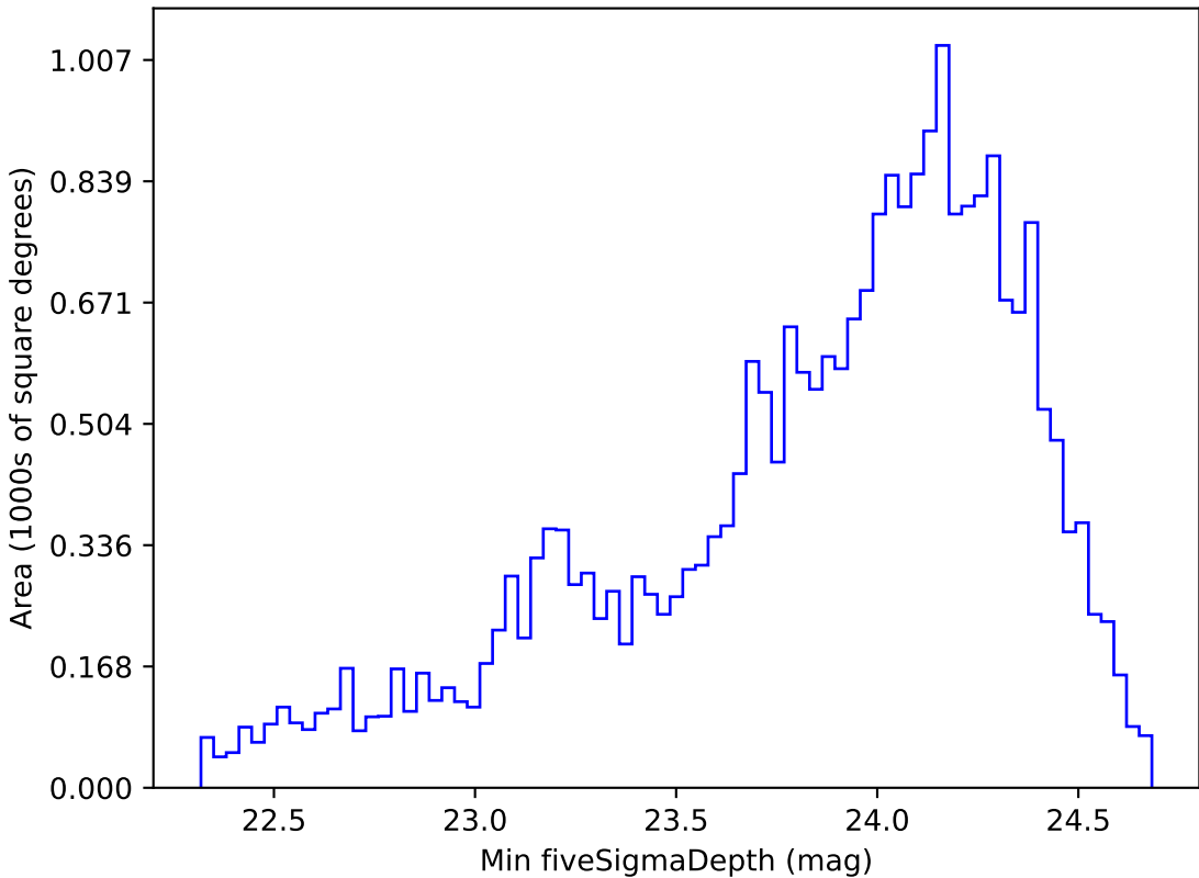
early_u_fpextra3.0_v3.4_10yrs Yr 1 g band: Min fiveSigmaDepth
