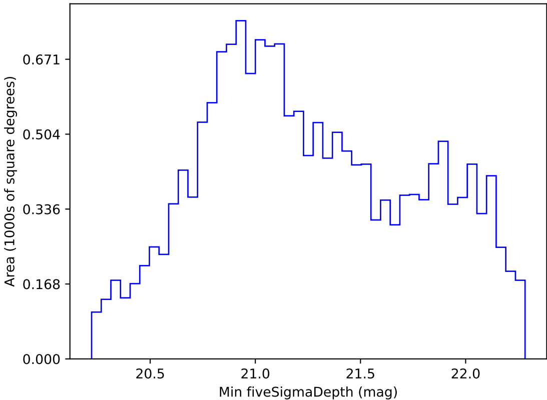
early_u_fpextra3.0_v3.4_10yrs WFD z band: Min fiveSigmaDepth
