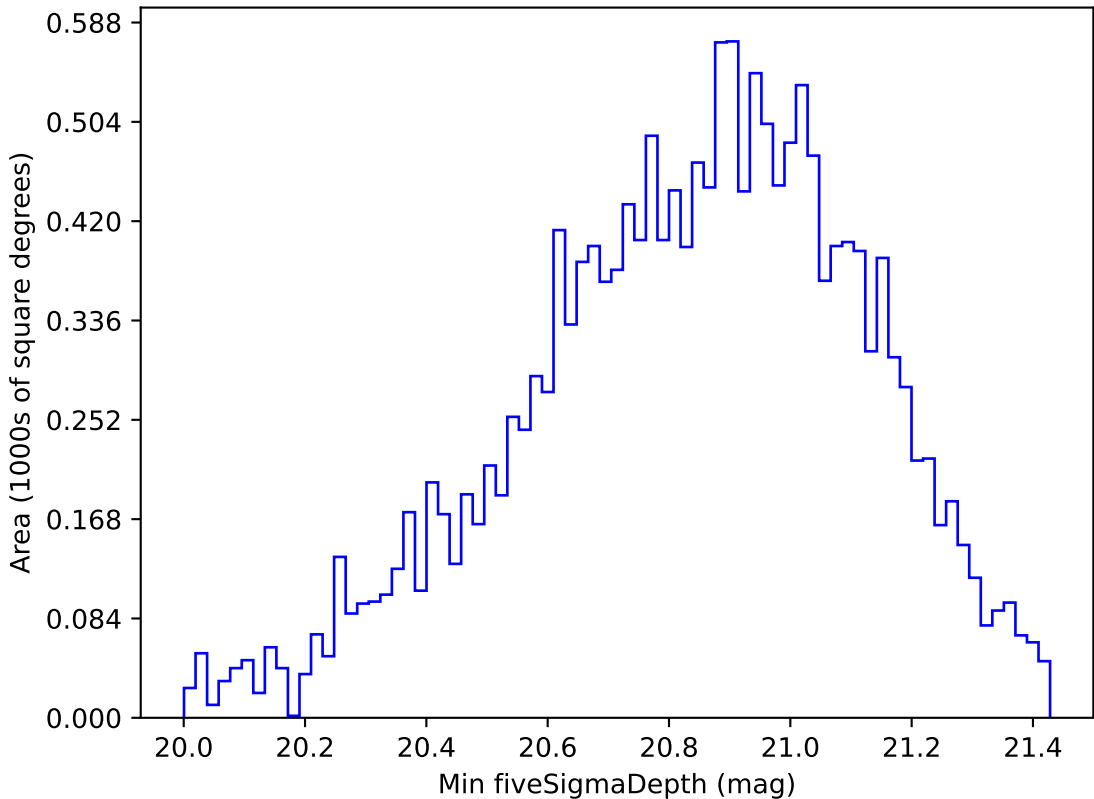
early_u_fpextra3.0_v3.4_10yrs WFD y band: Min fiveSigmaDepth
