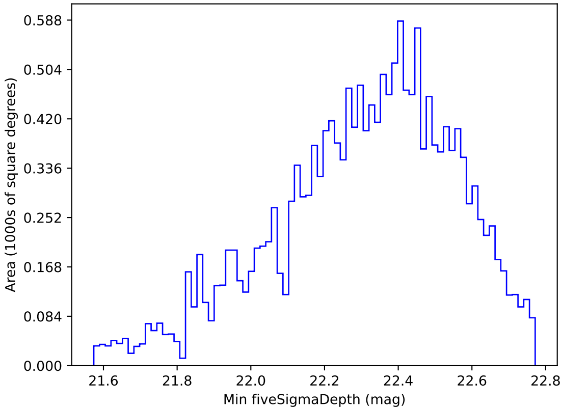
early_u_fpextra3.0_v3.4_10yrs WFD u band: Min fiveSigmaDepth
