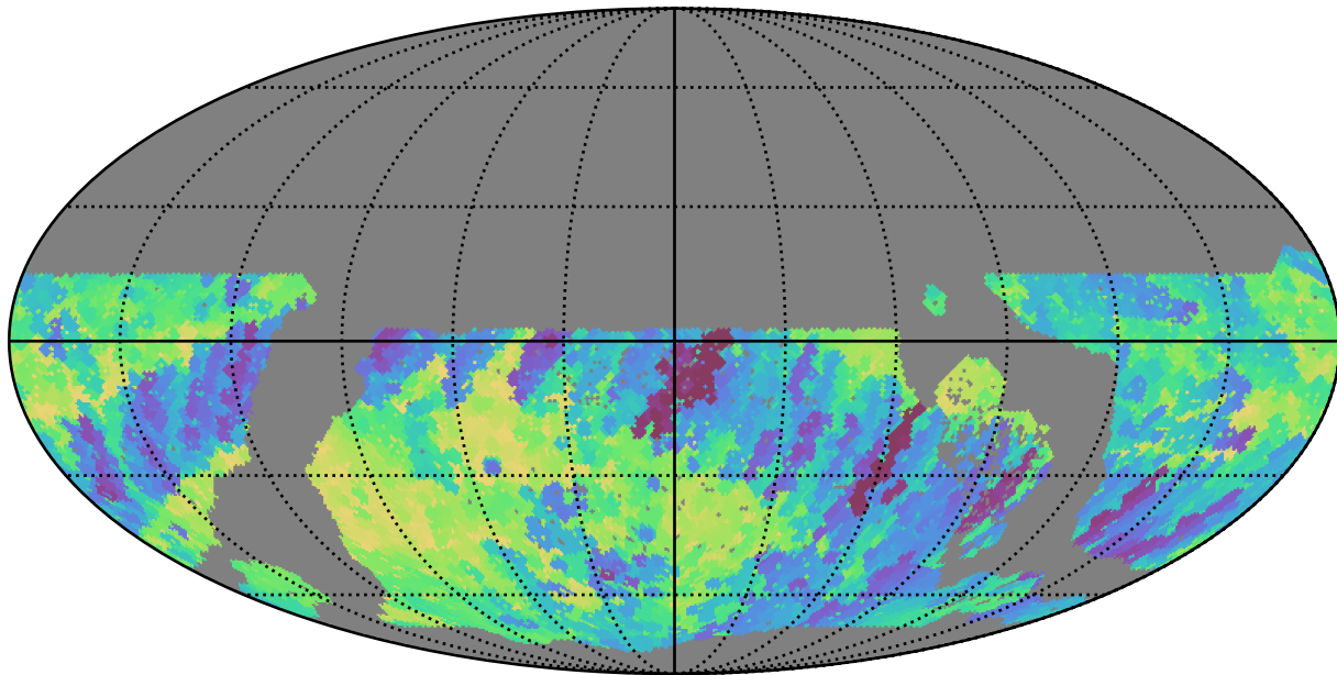
early_u_fpextra3.0_v3.4_10yrs WFD r band: Min fiveSigmaDepth
