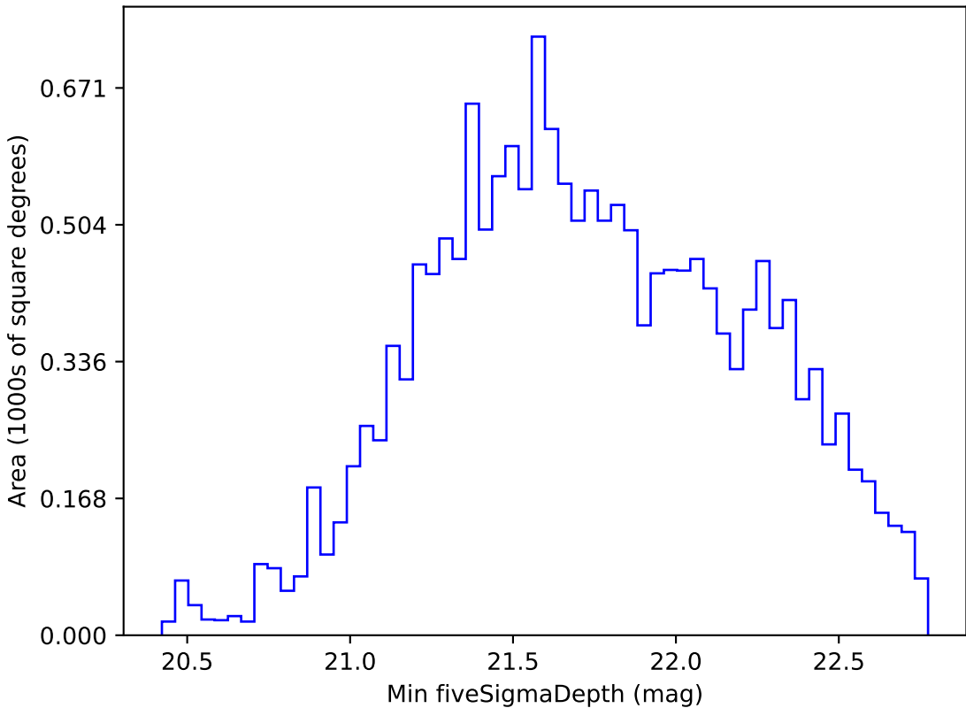
early_u_fpextra3.0_v3.4_10yrs WFD i band: Min fiveSigmaDepth
